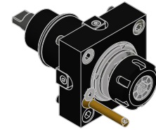
STRAIGHT DRILL-MILLING LIVE TOOL EXTERNAL NUT .....pg 39
