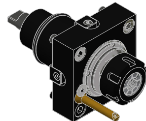
STRAIGHT DRILL-MILLING LIVE TOOL .....pg 15
