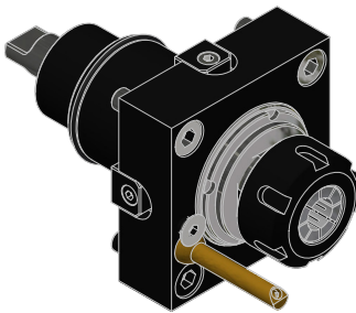
STRAIGHT DRILL-MILLING LIVE TOOL.....pg 57
