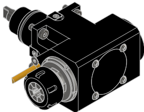
RIGHT ANGLE DRILL-MILLING LIVE TOOL EXTERNAL NUT .....pg 26
